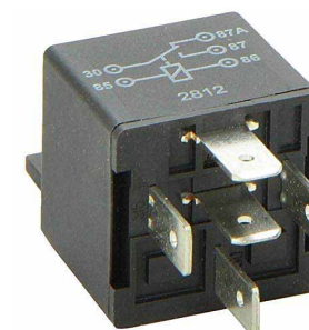
Standard Relay SPDT (Single Pole Double Throw)
